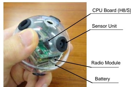
図 4: The Experimental Sensor Node
